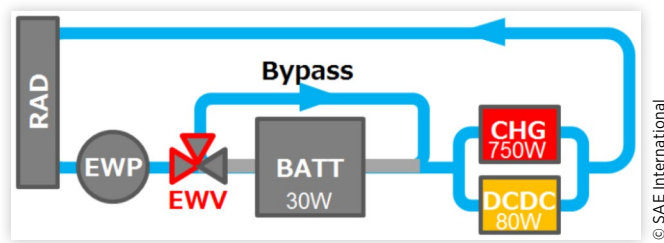
FIGURE 22 IPU cooling channel during charging (Bypass)
