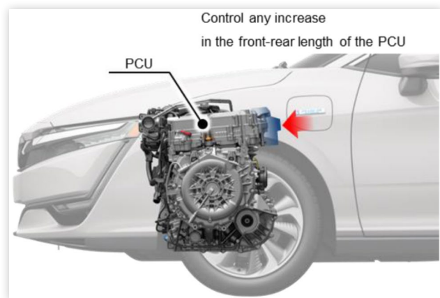
FIGURE 31 Power-plant layout in engine room
