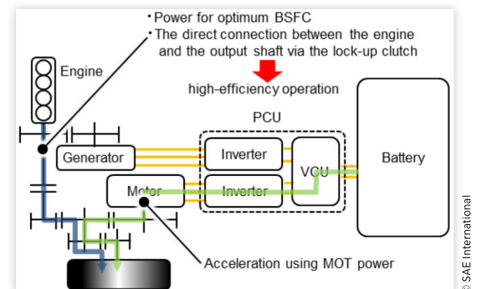
FIGURE 9 Overview of drive power output in Engine Driving Mode
