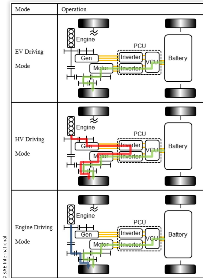
FIGURE 4 Powertrain operation
