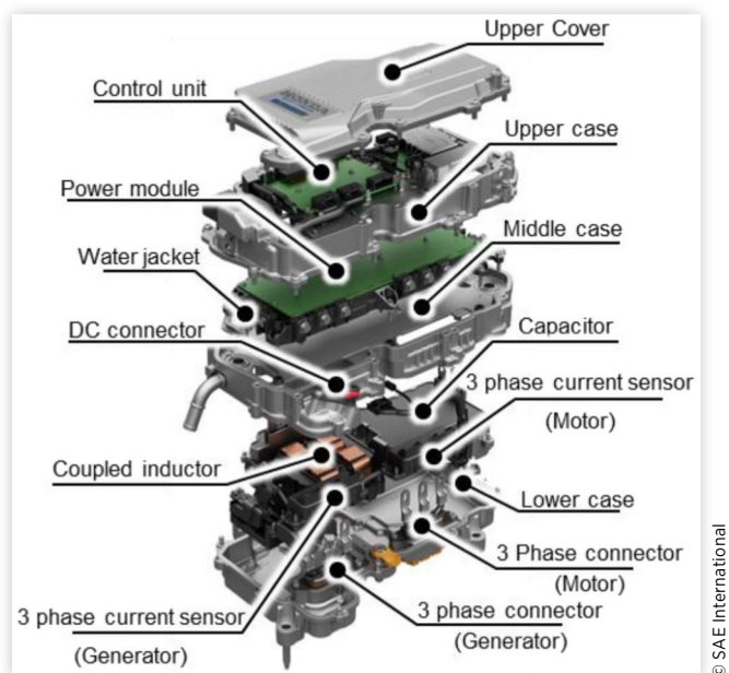
FIGURE 26 PCU configuration
