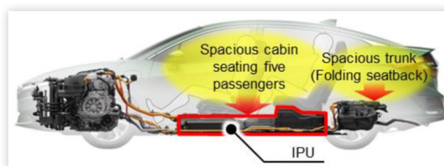
FIGURE 2 Side view of powertrain layout
