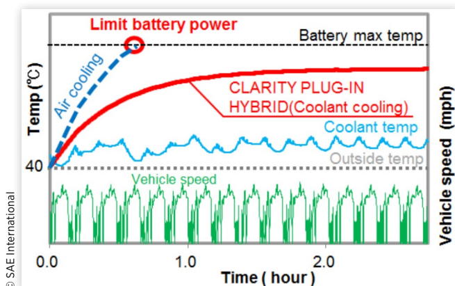
FIGURE 19 Battery temperature during high-load operation
