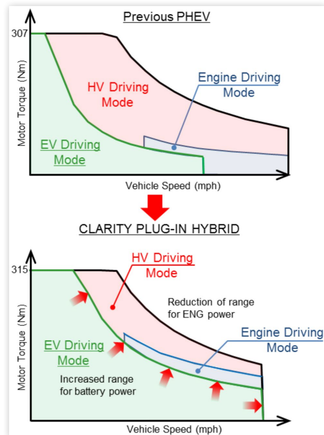
FIGURE 7 System operation at each vehicle speed and motor torque
