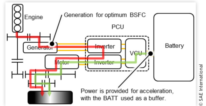
FIGURE 8 Relationship between power generated by the engine and battery power in HV Driving Mode
