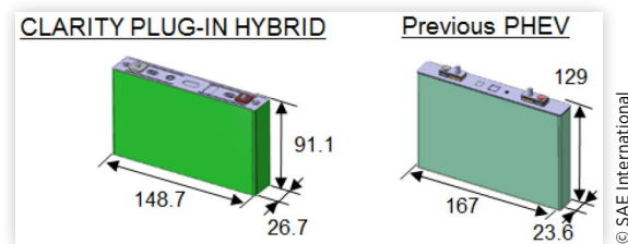
FIGURE 16 Cell size
