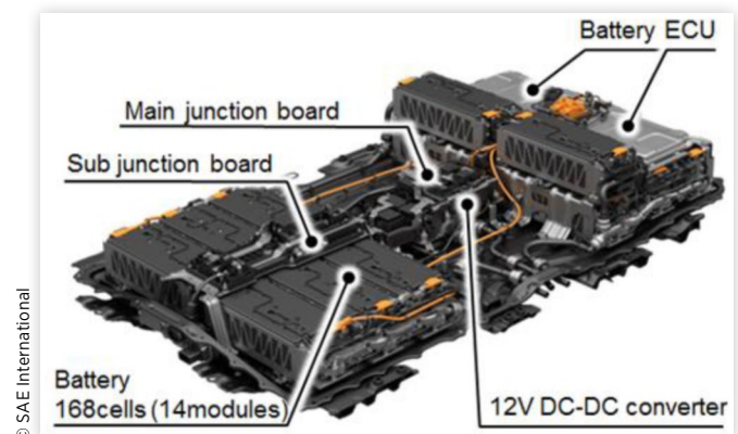
FIGURE 13 Layout of IPU components
