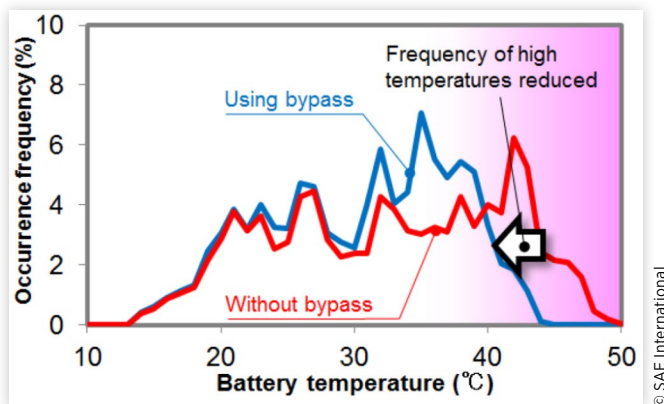
FIGURE 23 Bypass effect on frequency of battery temperature
