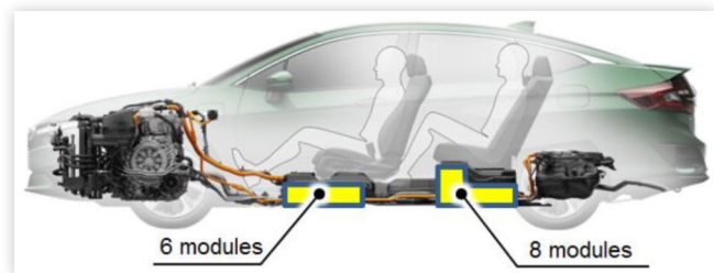
FIGURE 14 Powertrain side view of the CLARITY PLUG-IN HYBRID
