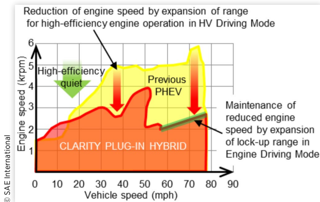
FIGURE 10 Frequency of engine speed at each vehicle speed during city and highway driving in CS operation
