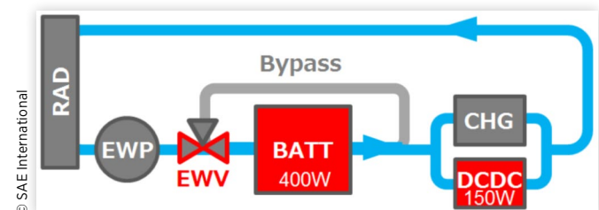
FIGURE 21 IPU cooling channel during vehicle operation (Main)
