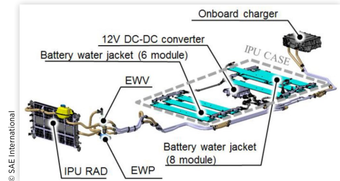
FIGURE 20 Components of IPU cooling circuit
