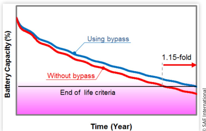
FIGURE 24 Bypass effect on deterioration of battery capacity
