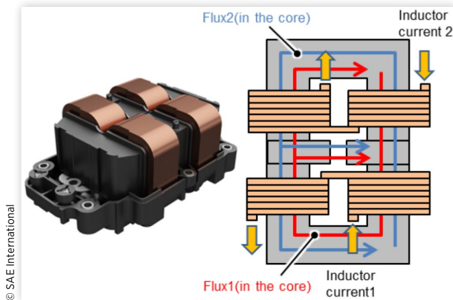
FIGURE 29 Coupled inductor configuration
